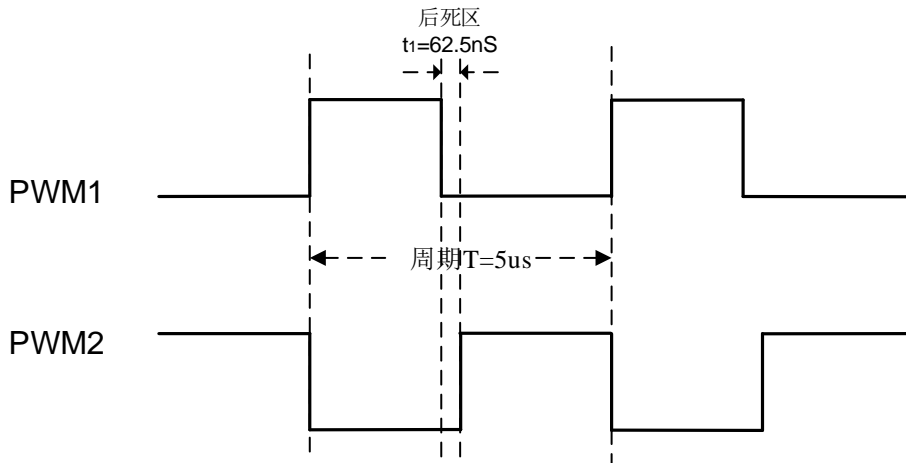
PWM1及PWM2输出波形图
