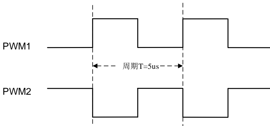
PWM1及PWM2输出波形图
