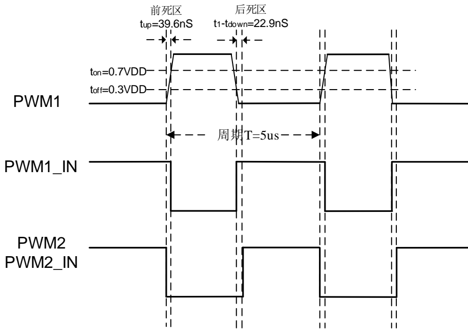
PWM1及PWM2输出波形图
