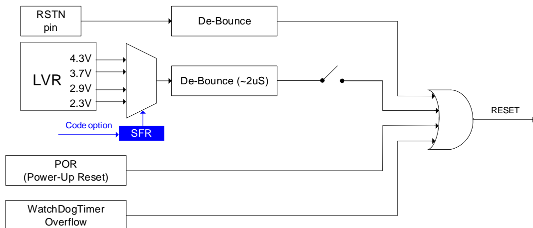
The SC92F827X Reset Diagram
