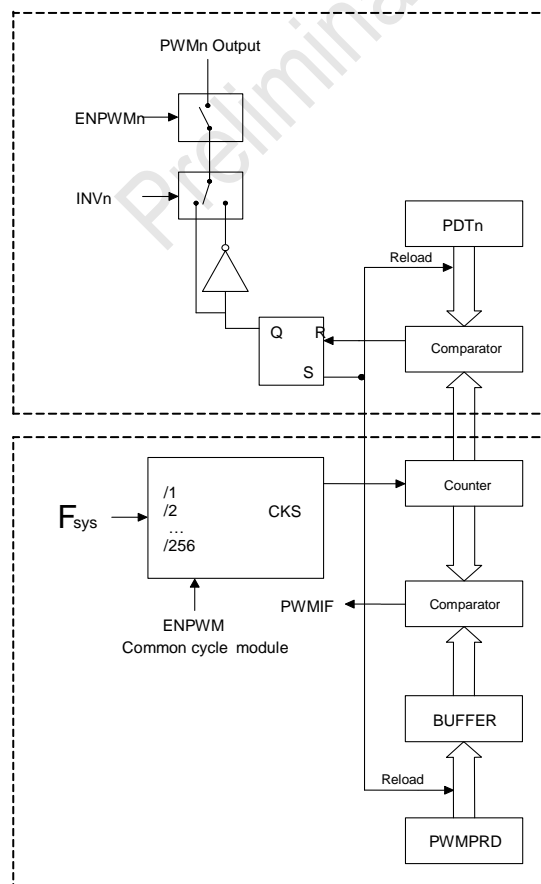
The SC92F827X PWM block Diagram
