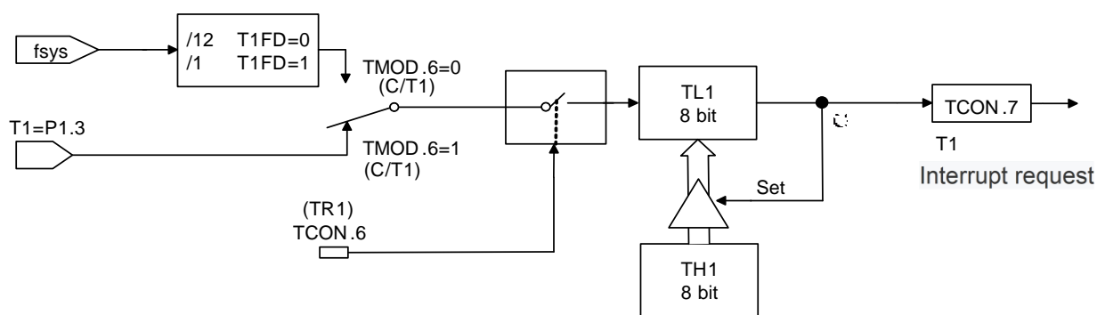
Operating Mode 2: 8bit Automatic Reload Counter/Timer
