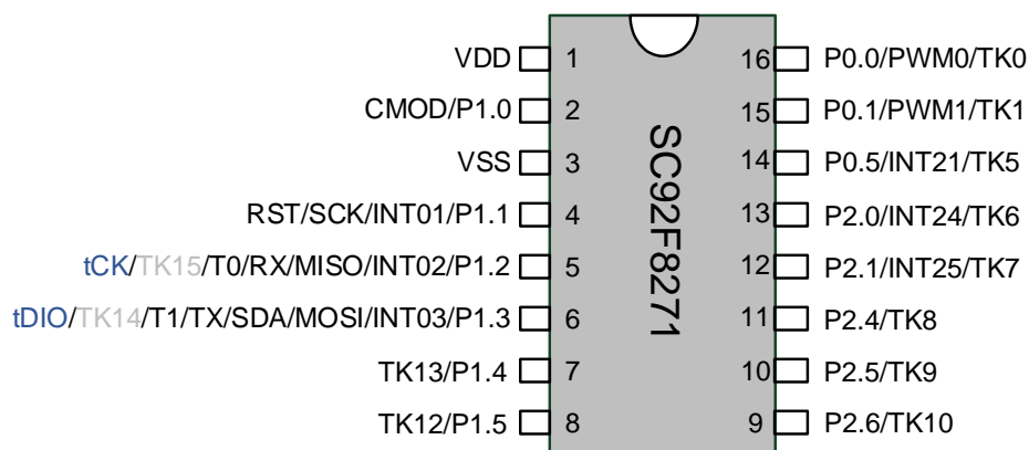
The SC92F8271 Pin Diagram
