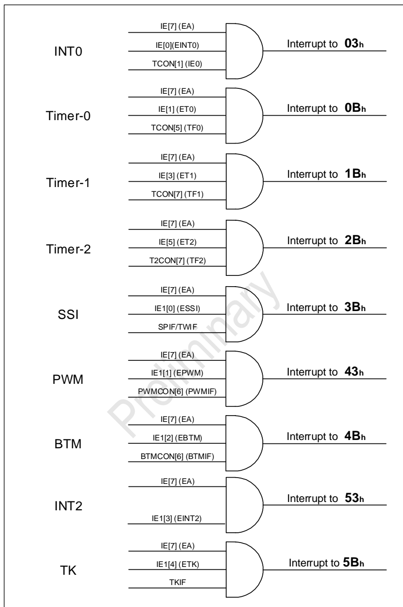
The SC92F827X Interrupt Structure and Vector
