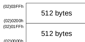
SC95FWXX 1 Kbytes LDROM Sector 示意
