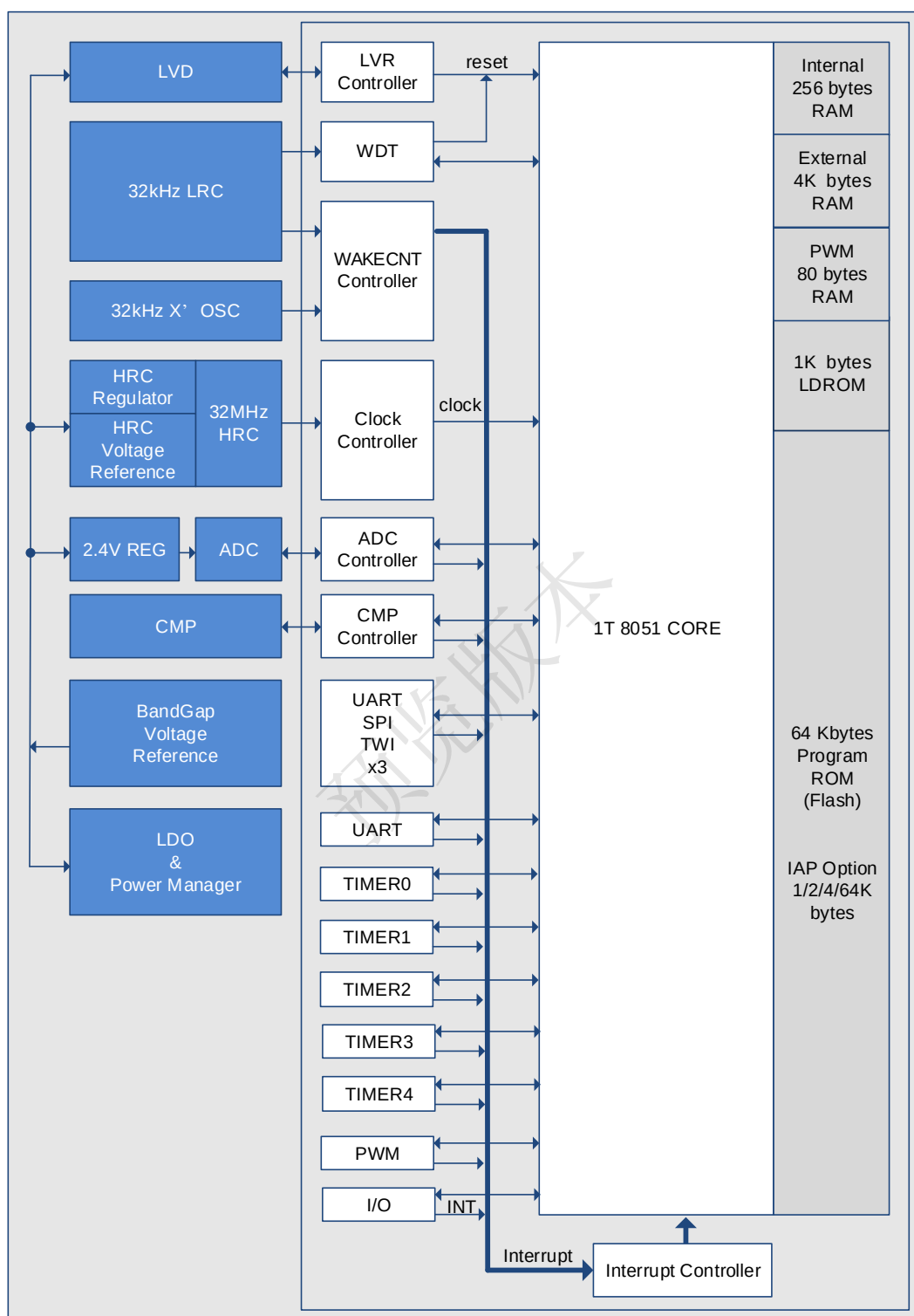
SC95FWXX BLOCK DIAGRAM
