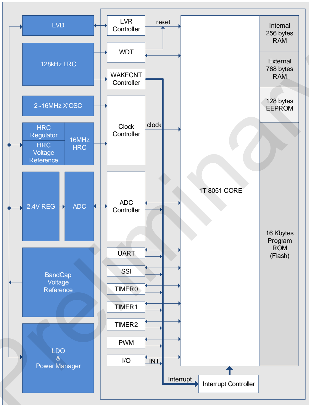
SC92F740X BLOCK DIAGRAM
