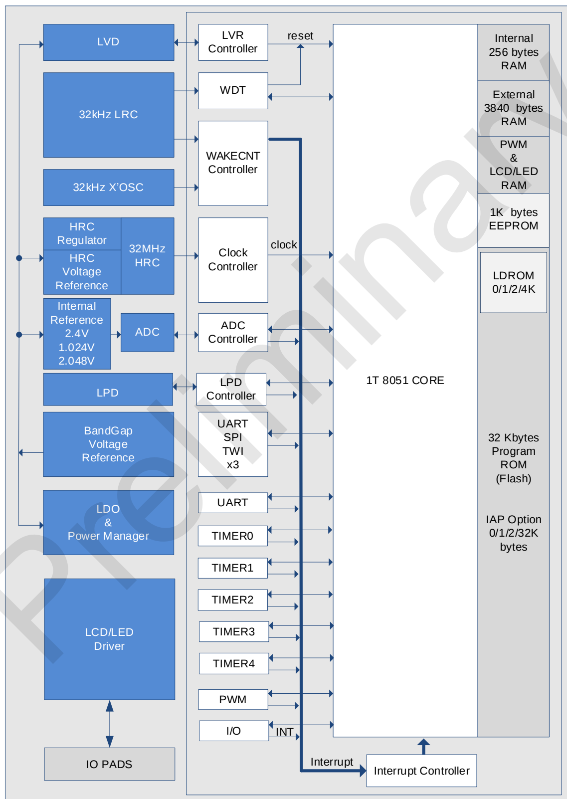
SC92L753X BLOCK DIAGRAM
