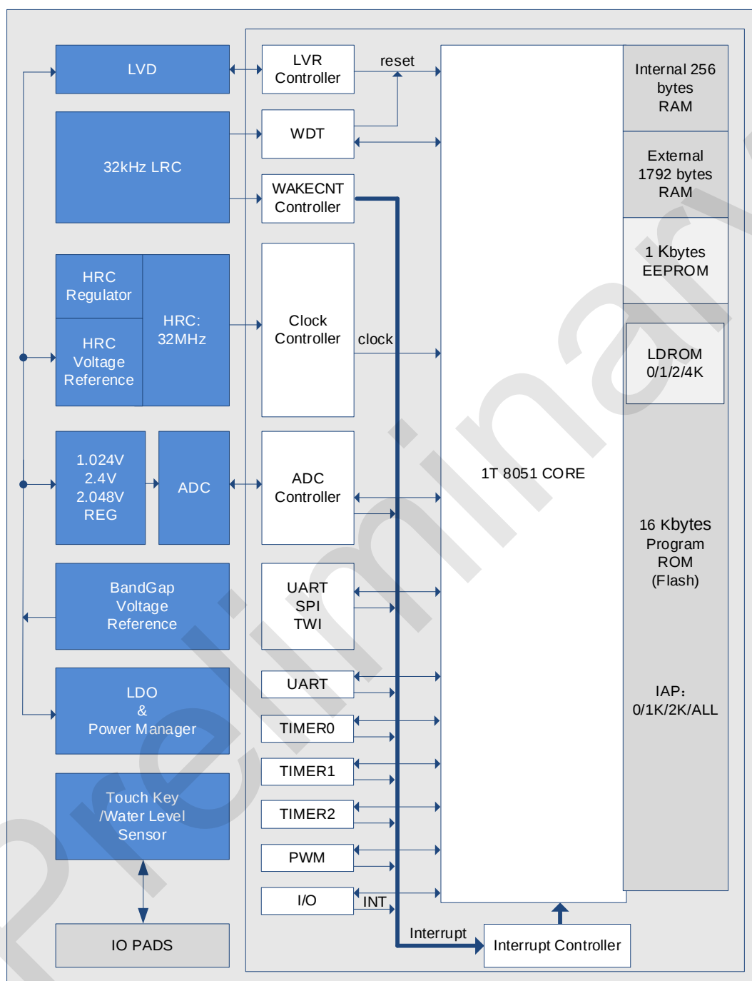
SC92R425 BLOCK DIAGRAM
